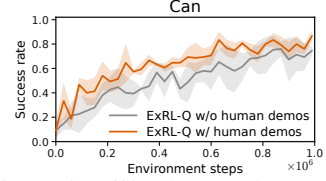
Figure 5: Offline human demonstrations improve early online adaptation of ExRL-Q on Can ( H = 50 ).
