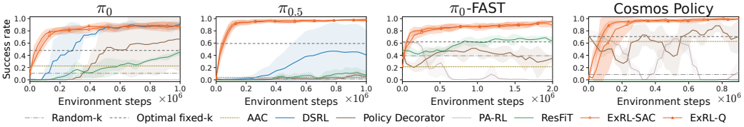
Figure 4: ExRL enables sample-efficient online adaptation of different classes of generalist robot policies on Libero, including the flow-based VLA models \pi_0 and \pi_{0.5} , the autoregressive VLA model \pi_0 -FAST, and the world action model Cosmos Policy. All base policies are of chunk size 50.
