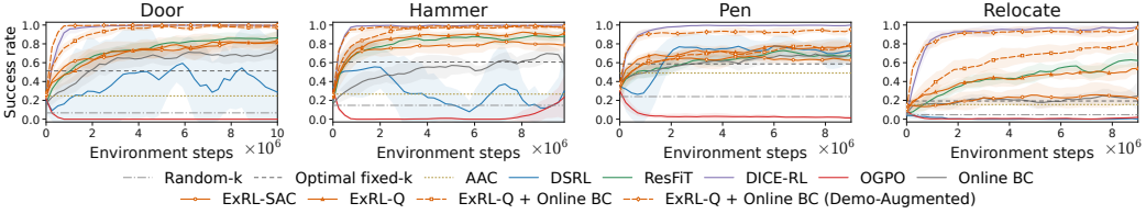
Figure 3: Online adaptation of DP on Adroit with chunk size H = 32 .
