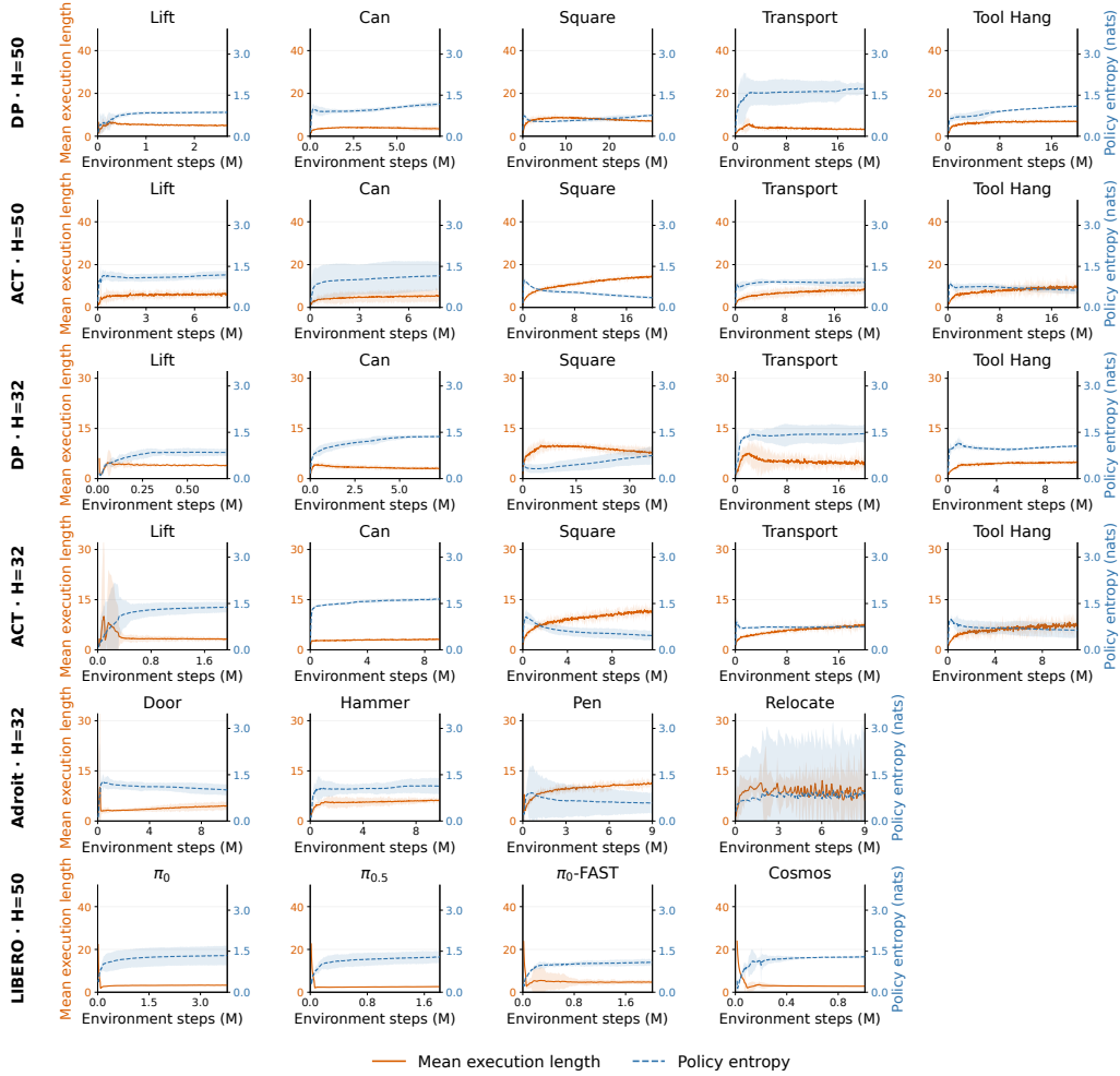
Figure 15: Evolution of execution lengths and policy entropy learned by ExRL-SAC. Orange solid curves show mean execution length; blue dashed curves show the categorical policy entropy on training minibatches. Shaded bands indicate 95% confidence intervals over three training seeds.
