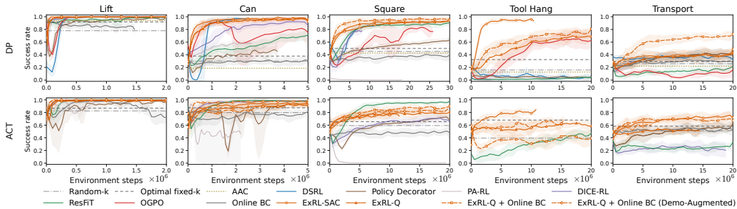
Figure 12: Online adaptation of DP and ACT on Robomimic with chunk size H = 32 .
