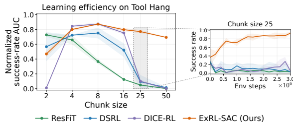
Figure 1: Prior RL methods are sample-inefficient when adapting diffusion policy with long action chunks. Left: Normalized success-rate AUC over the first 3M environment steps versus chunk size on the Robomimic Tool Hang task. Right: RL learning curves for chunk size 25.
