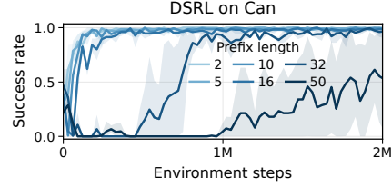
Figure 10: DSRL on Can. Three-seed means and 95% CIs. Prefixes 2–32 share an H = 32 checkpoint; prefix 50 uses an H = 50 checkpoint.
