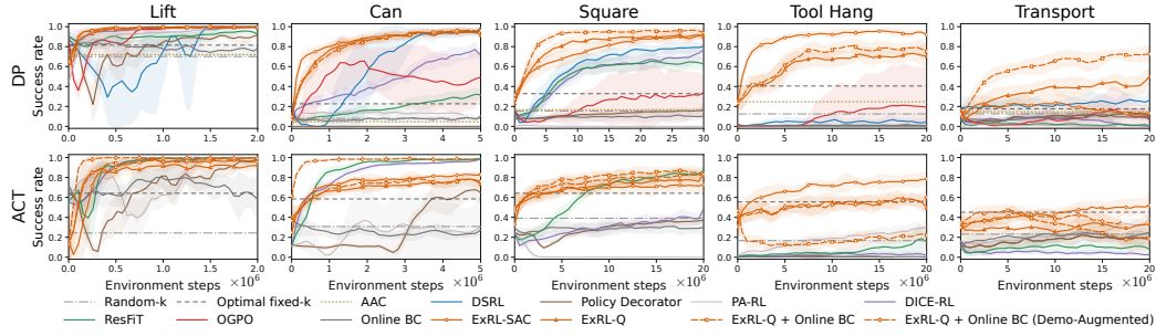
Figure 2: ExRL enables sample-efficient online adaptation of DP and ACT of chunk size 50 on Robomimic.
