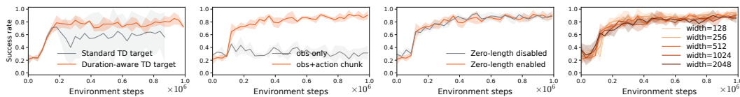
Figure 7: Ablation studies on Can with H = 32 . Left to right: duration-aware TD target, conditioning on the predicted action chunk, zero-length execution, and network width.
