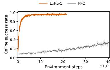
Figure 14: PPO versus ExRL-Q on Can. Mean online success over 200 episodes, with 95% CIs.
