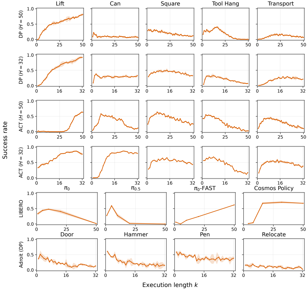
Figure 16: Fixed- k sweep across base policies and tasks. We evaluate each base policy under different fixed execution lengths on Robomimic, LIBERO, and Adroit. Performance varies substantially with k , and the optimal fixed execution length differs across tasks and policies, highlighting the importance of adaptive execution-length control. Shaded bands indicate 95% confidence intervals over three seeds.
