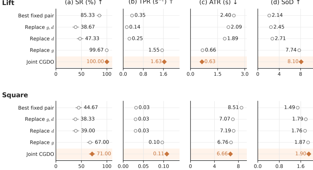
Figure 6: Replacing learned gain and duration with fixed averages. Duration replacement causes the larger losses. SR bars are 95% Wilson intervals. The unmodified study checkpoints achieve 100% SR/0.63 s ATR on Lift and 71%/6.66 s on Square .
