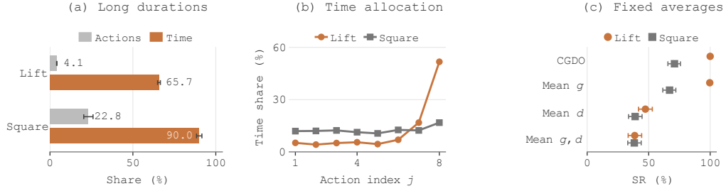
Figure 4: Learned gain-duration adaptation. (a) Shares of actions and execution time with d > 10 ms. (b) Time share by action index j within a chunk. (c) SR after fixing g , d , or both to their mean at each index, estimated from separate episodes, without retraining. Each task/condition uses 300 episodes; intervals are 95% episode-bootstrap in (a) and Wilson in (c).
