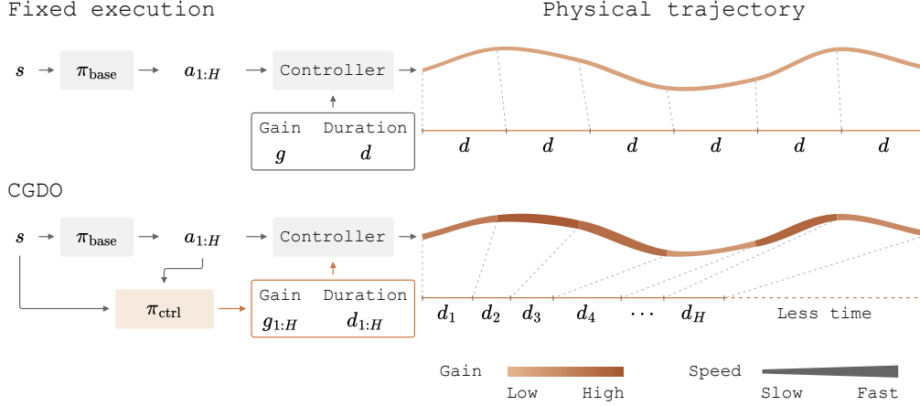
Figure 1: Coupled gain–duration optimization accelerates policy execution. Fixed execution (top) applies every predicted action with the same gain g and duration d . CGDO (bottom) keeps the base policy frozen and jointly adapts per-action gain and duration. Higher gain can drive the robot toward the current target faster, while shorter duration switches to the next action sooner; coordinating the two therefore allows the action sequence to be executed in less physical time.
