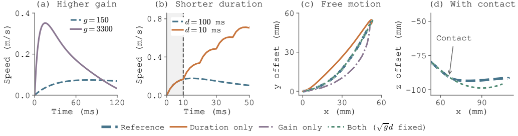
Figure 2: Gain–duration dynamics study. (a) Higher gain accelerates the initial speed. (b) Shorter duration reduces braking by advancing to the next target. (c) Either change alone alters the path; increasing gain and shortening duration with \sqrt{gd} fixed approximately preserves it at fourfold peak speed. (d) The same rule fails to preserve the path when a separate downward motion encounters soft contact.
