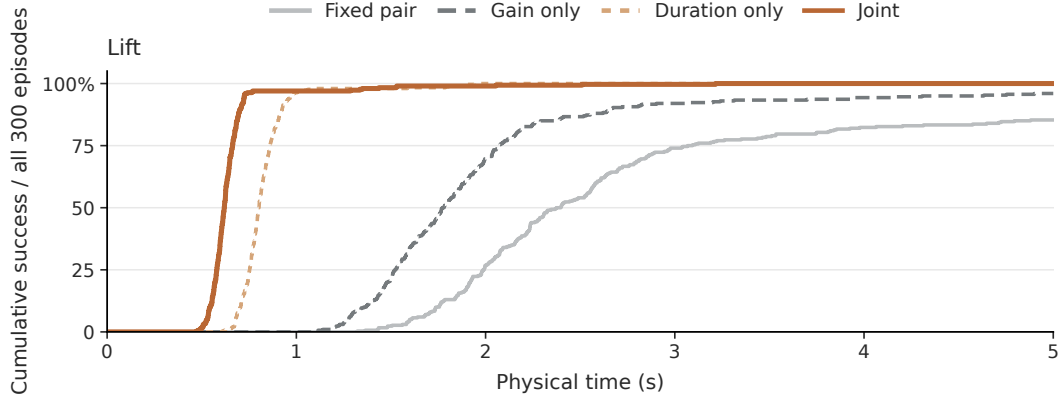
Figure 5: Success by elapsed time. All 300 episodes contribute to each curve, including failures. Controllers and initial states match Table 12.
