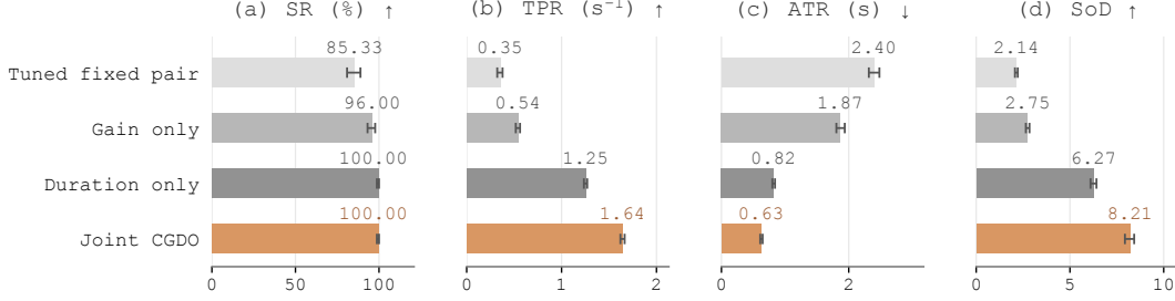
Figure 3: Learning gain and duration together performs best.
